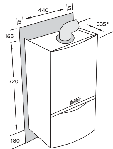
*369mm - ecoTEC plus 630
